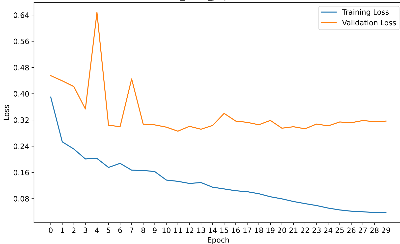
UBFC_UBFC_physnet Losses
